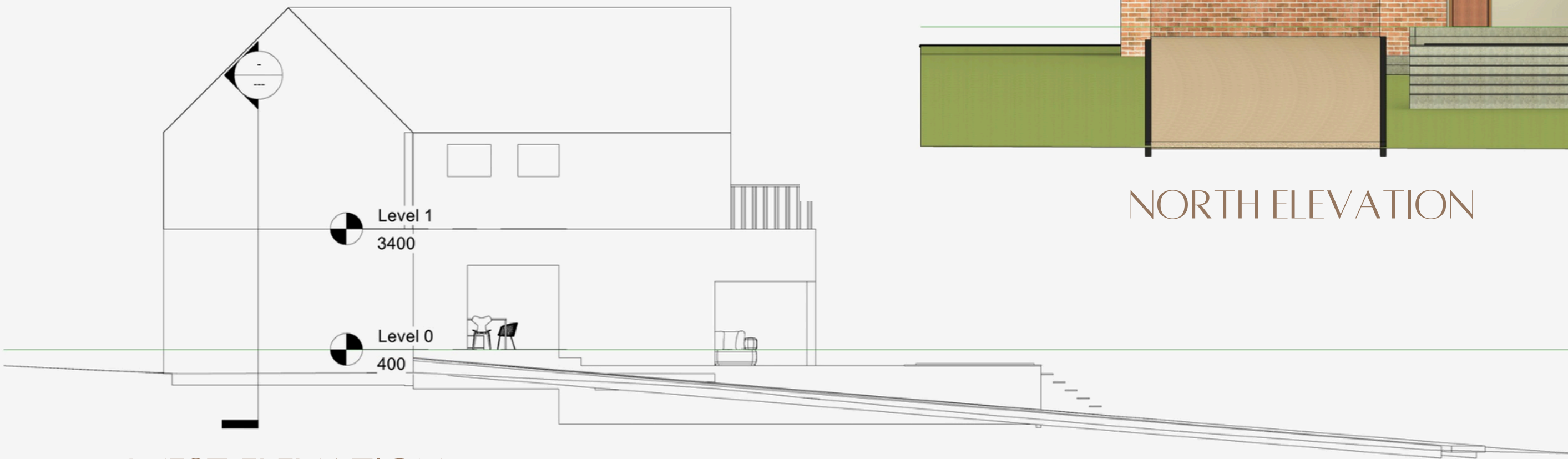
WEST ELEVATION
